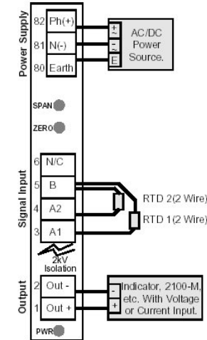
XJ4-N Differential RTD Input. Connection Example.
