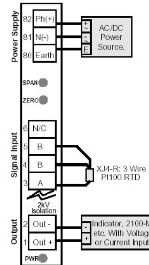
XJ4-R RTD Input. Connection Example.
